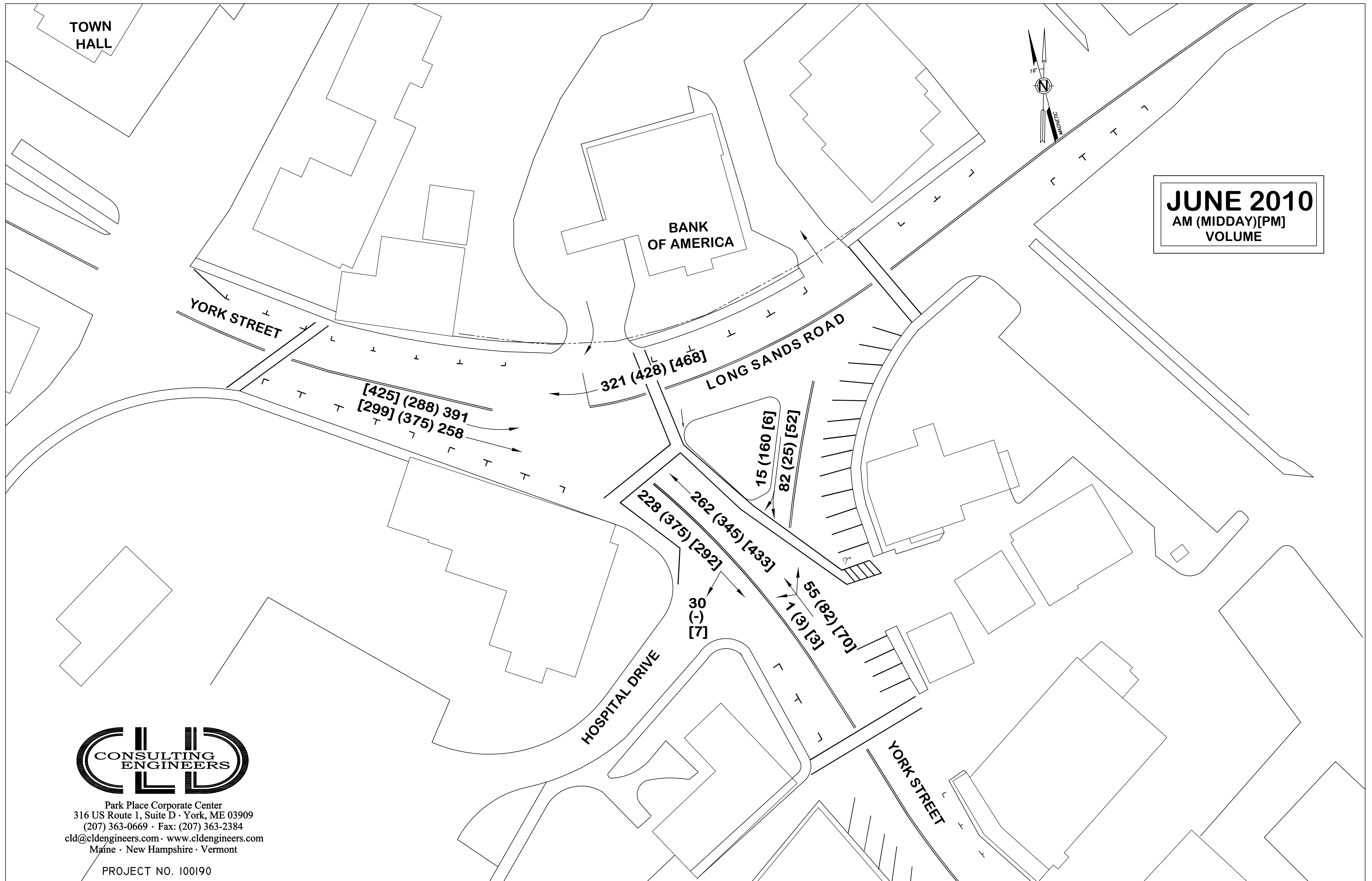
FIGURE 2: INTERSECTION TURNING MOVEMENT VOLUMES
